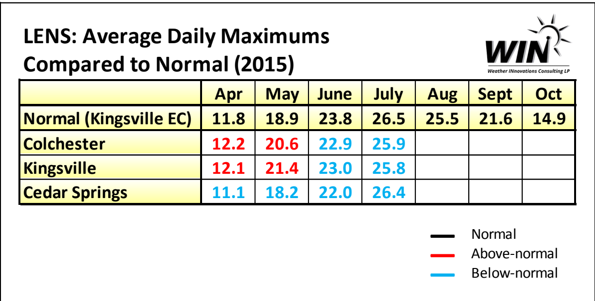
Figure 2: Maximum Temperatures
