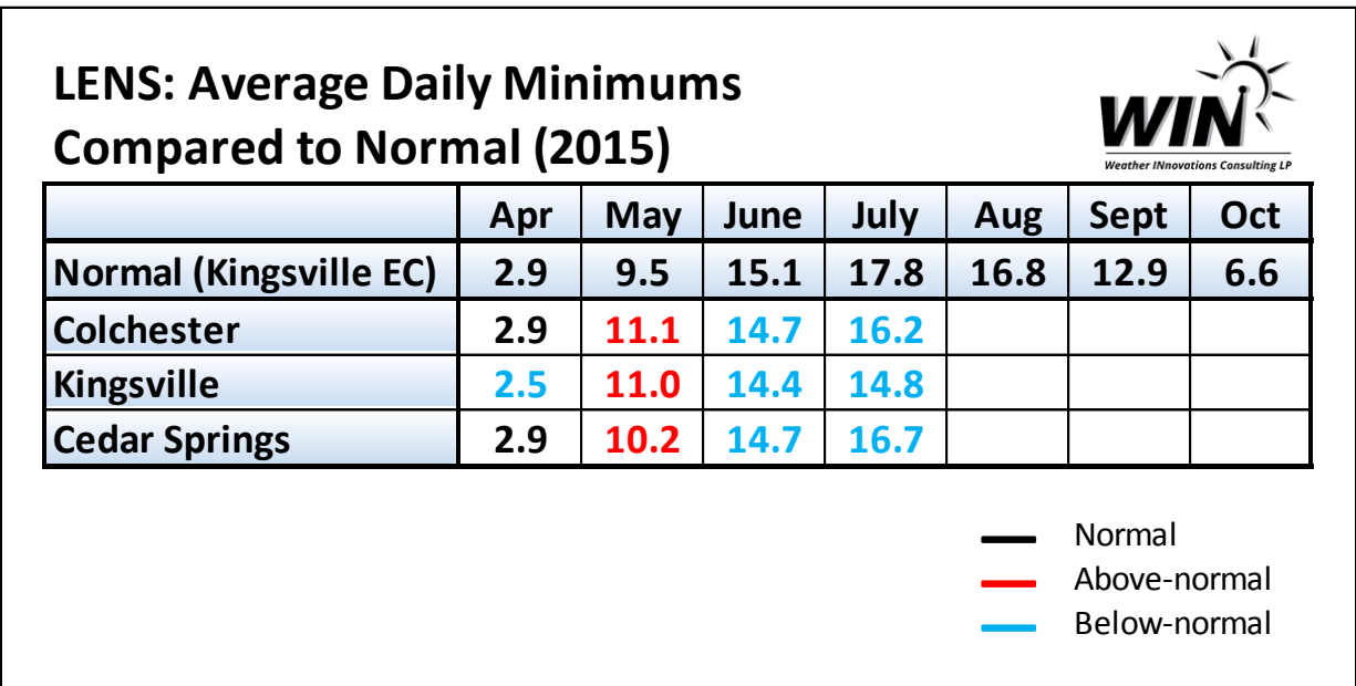
Figure 3: Minimum Temperatures
